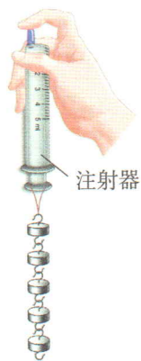
图8-28 估测大气压
